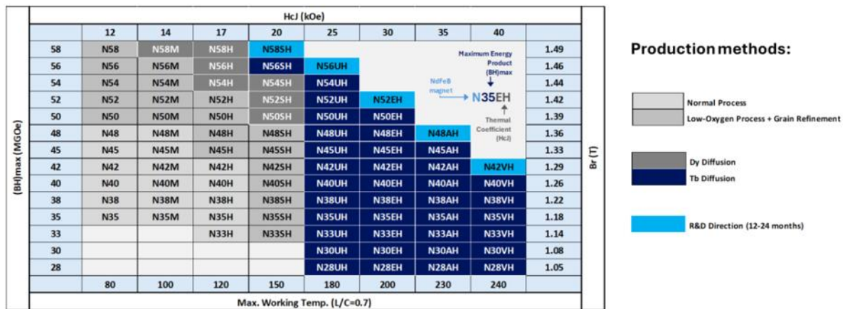
Figure 19.11 – High-temperature and high-strength grades of NdFeB often contain appreciable dysprosium and/or terbium
