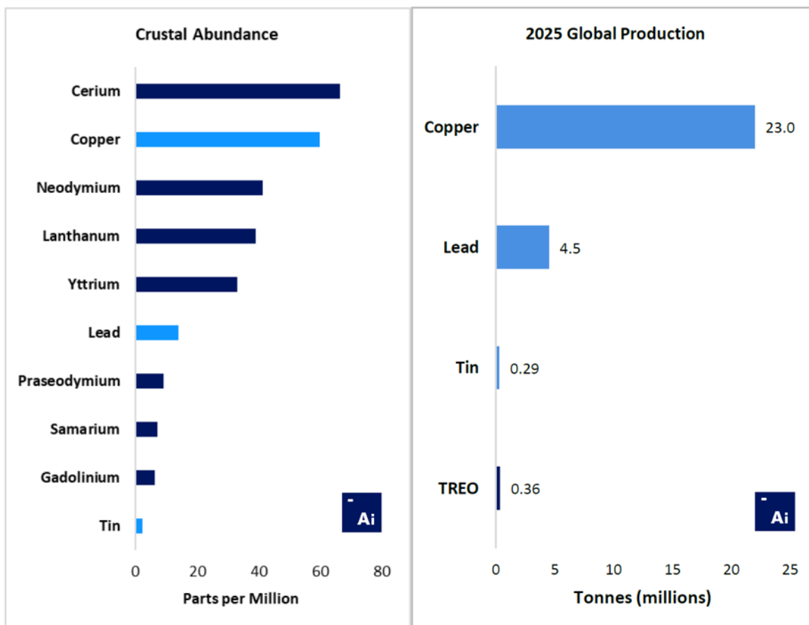
Figure 19.2 – Global production of REEs is remarkably low compared to similarly abundant éléments
