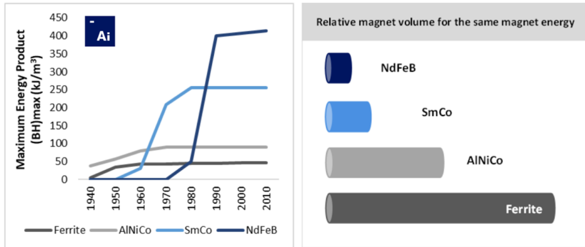
Figure 19.10 – NdFeB is the strongest permanent magnet material commercially available today
