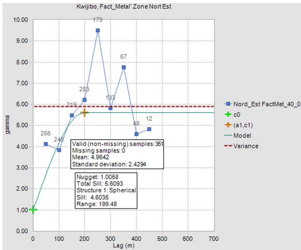
Figure 14.6 – Variogramme directionnel N40°
